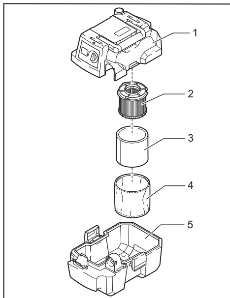
► 1. Tank cover 2. HEPA filter 3. Damper 4. Prefilter 5. Tank
